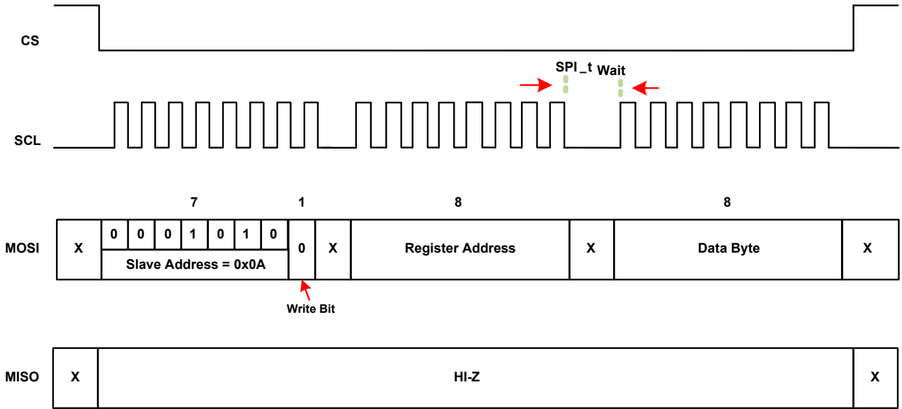
Figure 117. SPI Write
