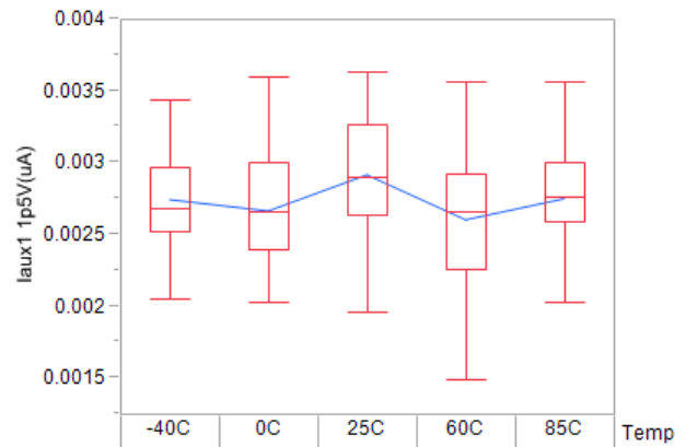
Figure 26. AUX1/xT1 Pin Input Current at 1.5V
