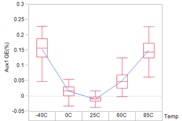
Figure 22. AUX1/xT1 Gain Error
