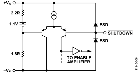
Figure 53. Shutdown Circuit
