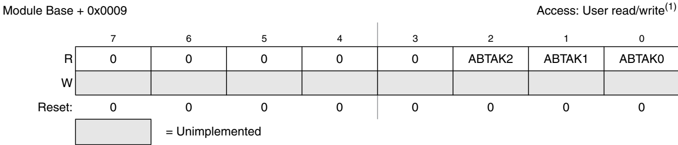
Figure 16-13. MSCAN Transmitter Message Abort Acknowledge Register (CANTAABK)
