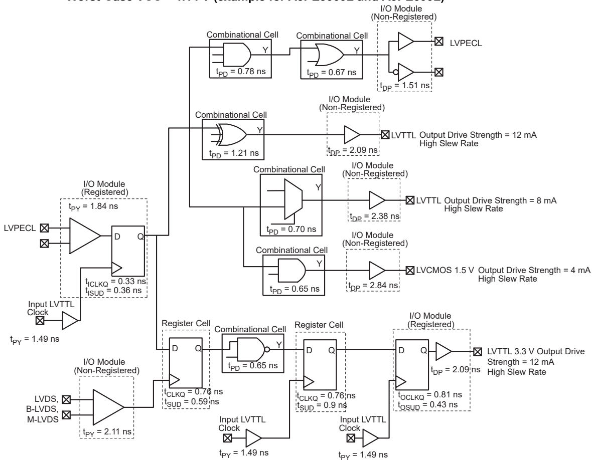
Figure 8 • Timing Model Operating Conditions: –1 Speed, Military Temperature Range ( T_J = 125^\circ\text{C} ), Worst-Case V_{CC} = 1.14\text{ V} (example for A3PE3000L and A3PE600L)
