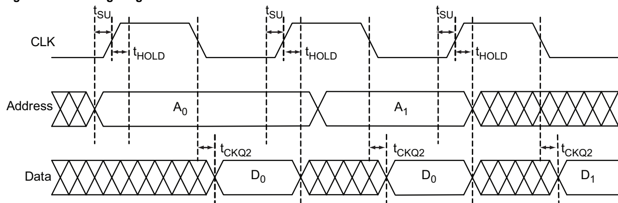
Figure 60 • Timing Diagram
