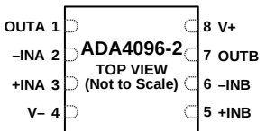
Figure 5. 8-Lead LFCSP (CP-8-10), ADA4096-2
