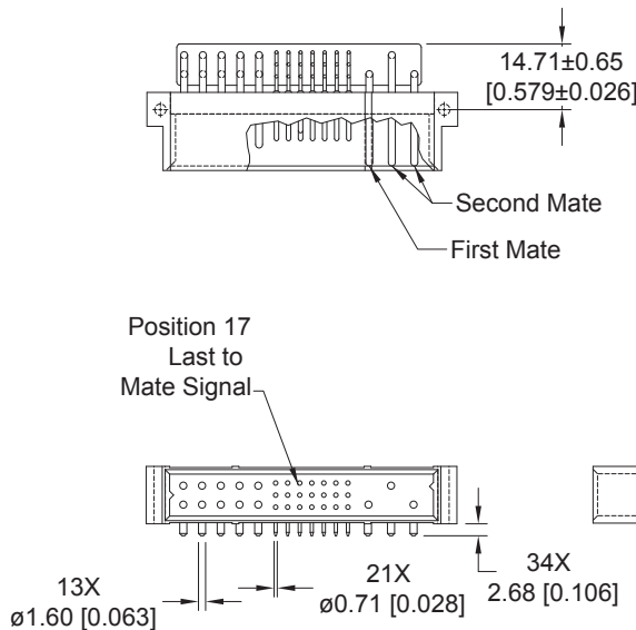
CONNECTOR DIMENSIONS
