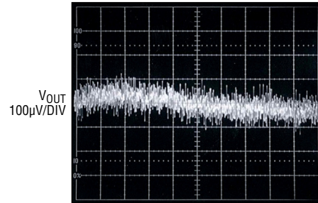
5V 10Hz to 100kHz Output Noise C_{REF/BYP} = 10\text{nF} , C_{FF} = 10\text{nF}
