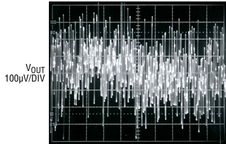
5V 10Hz to 100kHz Output Noise C_{REF/BYP} = 10\text{nF} , C_{FF} = 0
