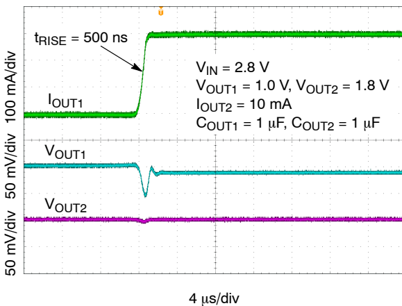
Figure 40. Load Transient Response – 1.0 V – Rising Edge, I_{OUT1} = 100\text{ μA} to 300\text{ mA}
