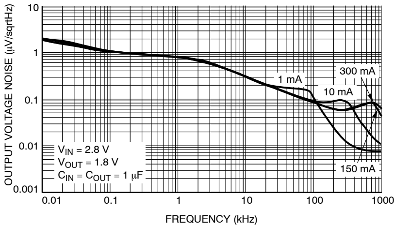
Figure 28. Output Voltage Noise Spectral Density for V_{OUT} = 1.8\text{ V} , C_{OUT} = 1\text{ }\mu\text{F}
