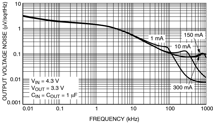
Figure 29. Output Voltage Noise Spectral Density for V_{OUT} = 3.3\text{ V} , C_{OUT} = 1\text{ }\mu\text{F}
