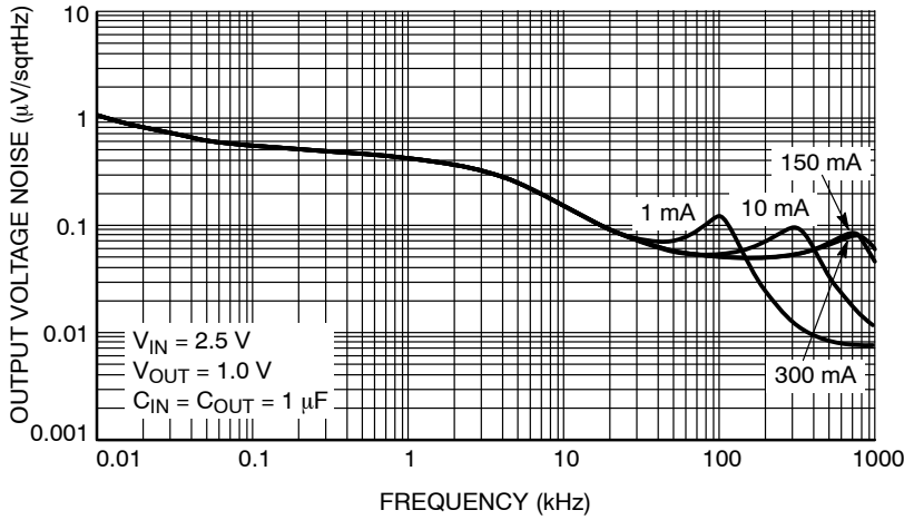
Figure 27. Output Voltage Noise Spectral Density for V_{OUT} = 1.0\text{ V} , C_{OUT} = 1\text{ }\mu\text{F}
