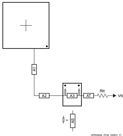
Figure 8-17. ADDR_CTRL Routing for Two Mirrored DDR3 Devices
