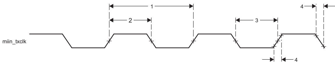
Figure 7-52. Clock Timing (GMAC Transmit) - MII operation
