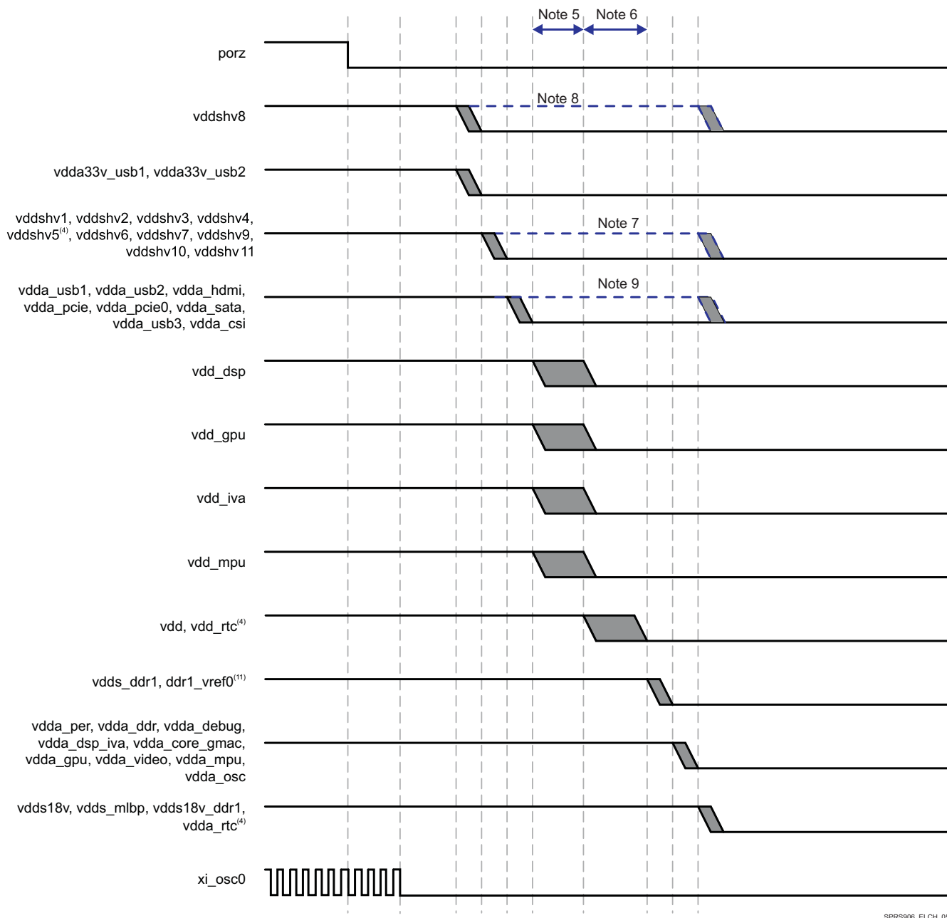
Figure 5-3. Power-Down Sequencing (10)(12)
