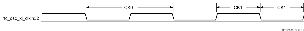
Figure 6-13. rtc_osc_xi_clkin32 Input Clock
