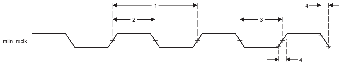
Figure 7-51. Clock Timing (GMAC Receive) - MII operation
