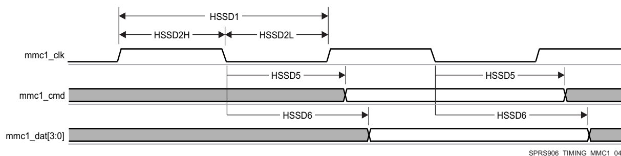
Figure 7-63. MMC/SD/SDIO in - High Speed - Transmitter Mode
