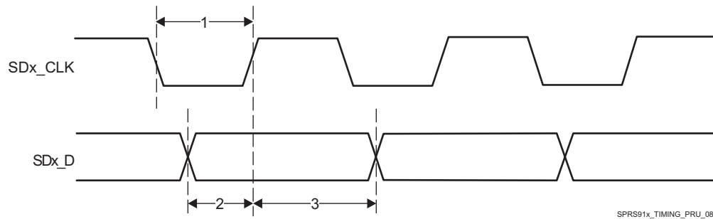
Figure 7-98. PRU-ICSS PRU SD_CLK Rising Active Edge
