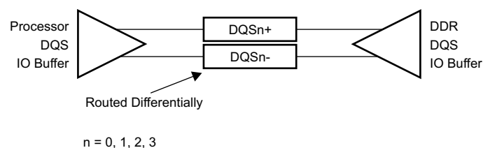
Figure 8-22. DQS Topology
