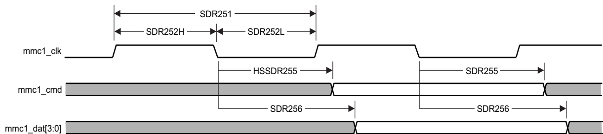
Figure 7-67. MMC/SD/SDIO in - High Speed SDR25 - Transmitter Mode
