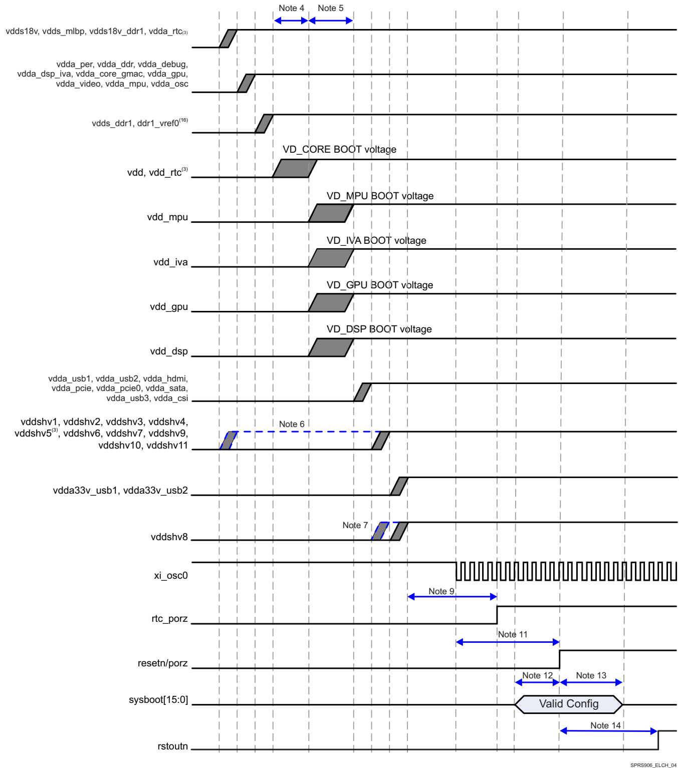
Figure 5-2. Power-Up Sequencing
