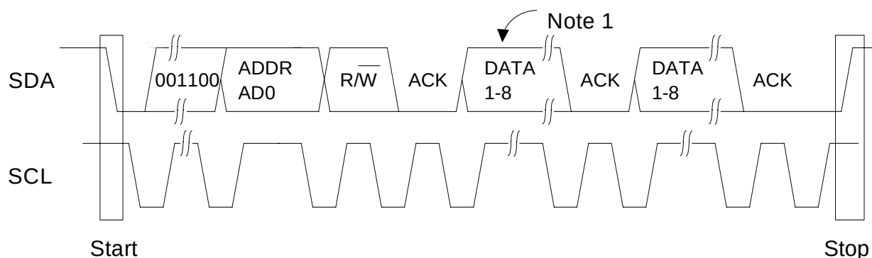
Figure 3. Control Port Timing - I 2 C Format
