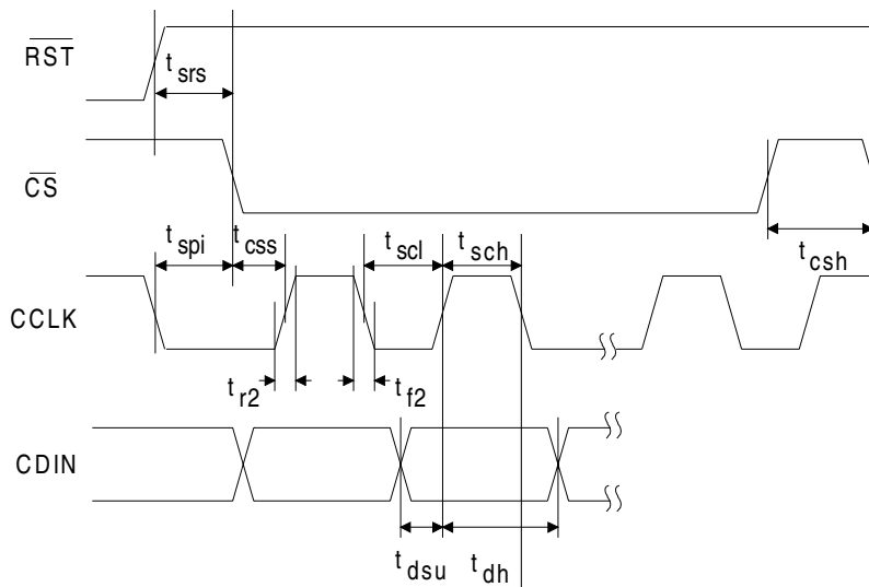
Figure 39. SPI Control Port Timing
