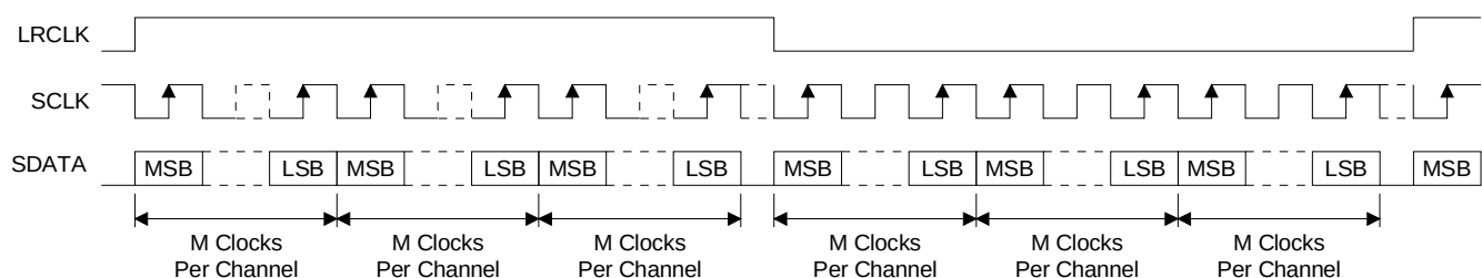
Figure 45. Multichannel Format
