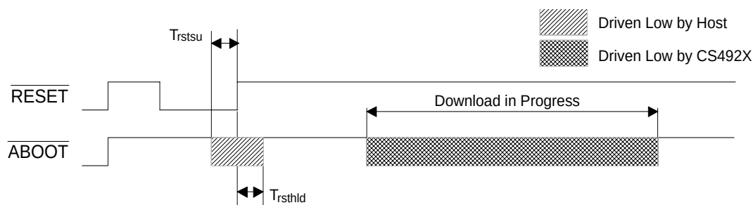
Figure 37. Autoboot INTREQ Behavior
