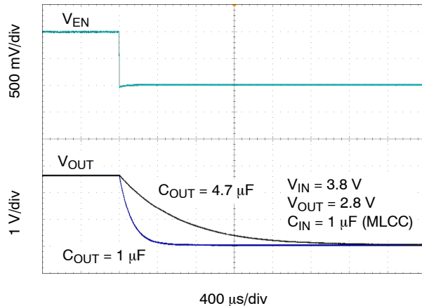
Figure 37. Enable Turn-off
