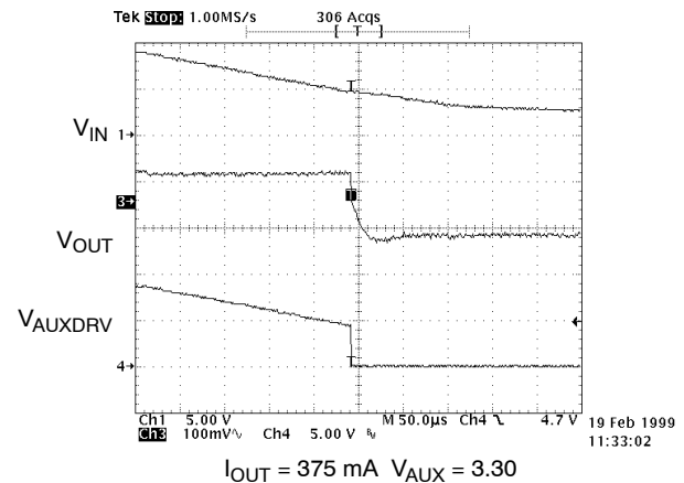
Figure 15. Power-Down, V_{AUX} = 3.3 V. Again, Note \Delta V = I R_{DS(ON)} \approx 130 mV
