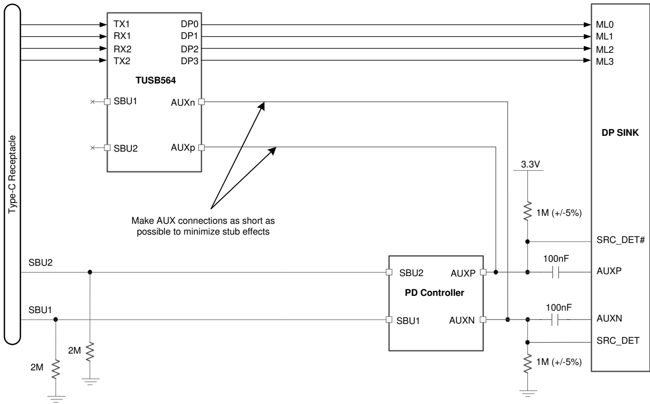
Figure 9-4. DisplayPort AUX Connections for UFP_D Pin Assignment E with External AUX Switching
