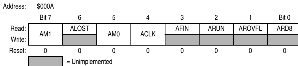
Figure 14-19. ESCI Arbiter Control Register (SCICTL)
