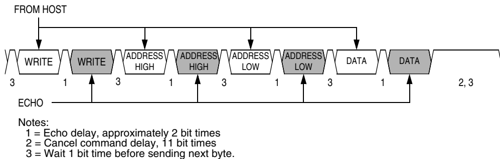
Figure 19-15. Write Transaction
