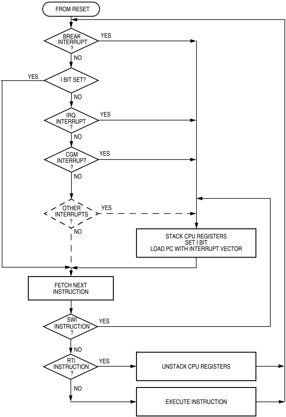
Figure 13-5. Interrupt Processing
