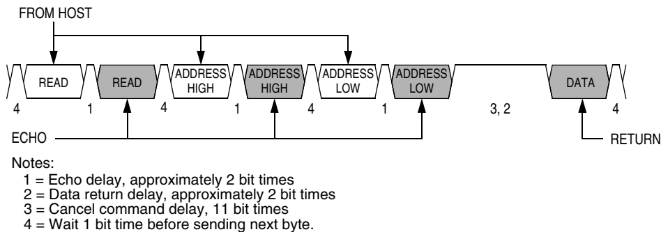
Figure 19-14. Read Transaction
