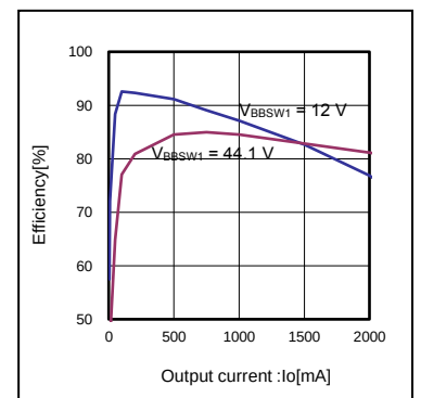
Figure 23. SWREG1 Efficiency-1 (5.0 V setting, Ta = 25 °C)
