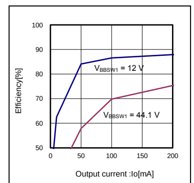
Figure 26. SWREG1 Efficiency-2 (3.3 V setting, Ta = 25 °C)
