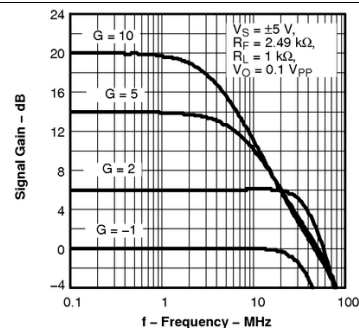
Figure 20. Frequency Response
