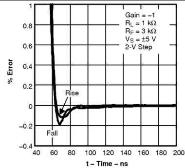
Figure 38. Settling Time
