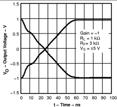
Figure 37. Settling Time
