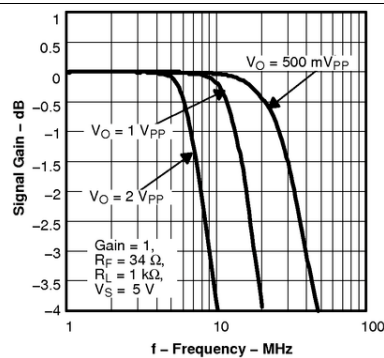
Figure 21. Frequency Response
