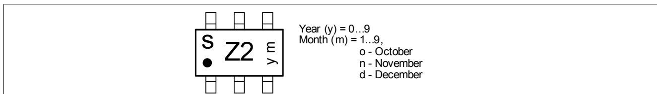
Figure 5 Marking PG-TSOP6-6-5
