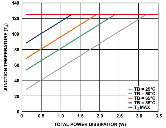
Figure 78. SOIC
