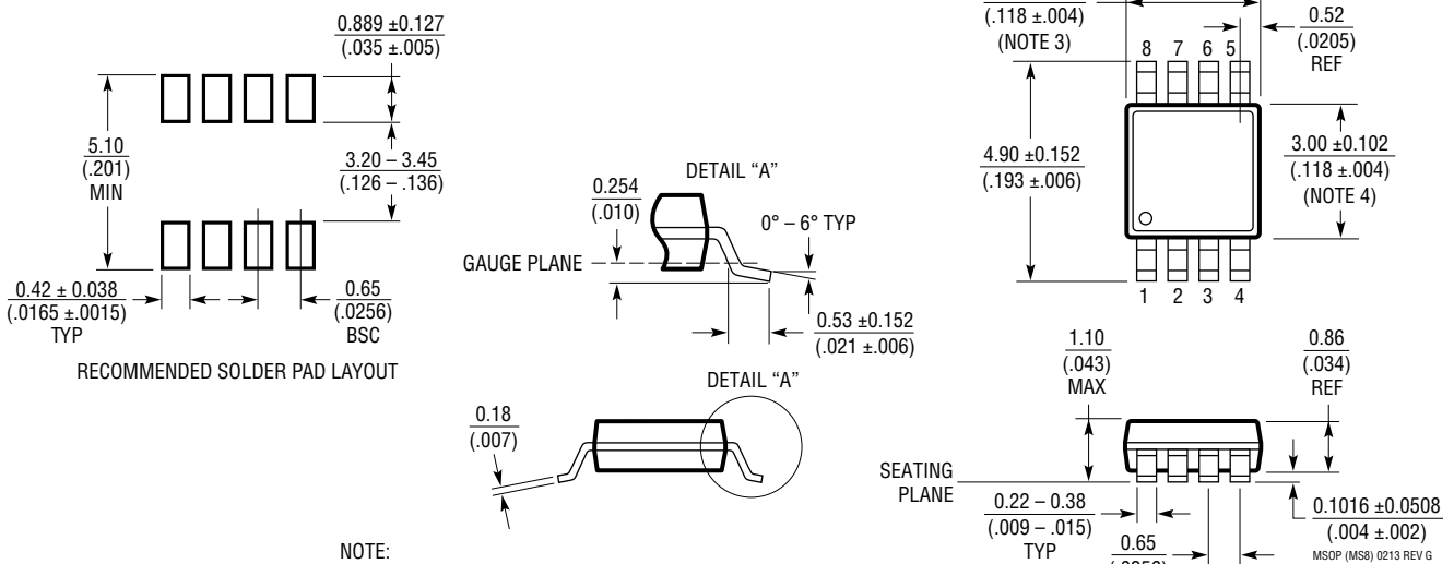
MS8 Package 8-Lead Plastic MSOP (Reference LTC DWG # 05-08-1660 Rev G)
