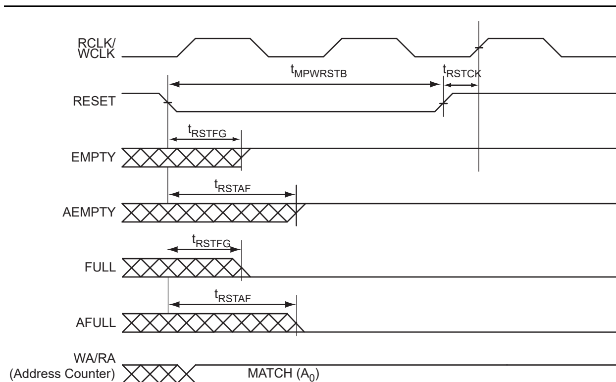
Figure 2-32 • FIFO Reset
