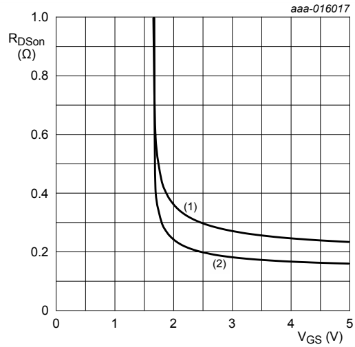
Fig. 10. Drain-source on-state resistance as a function of gate-source voltage; typical values I_D = 0.2\text{ A} (1) T_j = 150\text{ }^\circ\text{C} (2) T_j = 25\text{ }^\circ\text{C}
