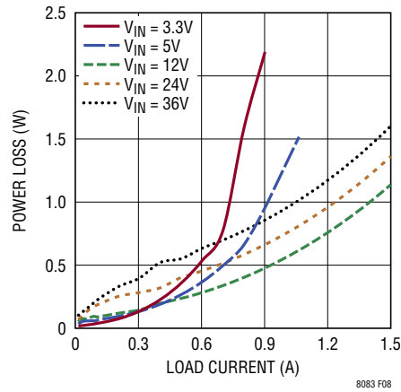
Figure 8. Power Loss at 5V OUT
