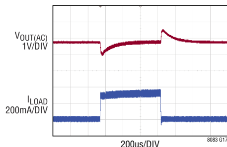
Transient Response from 18V IN to 36V OUT
