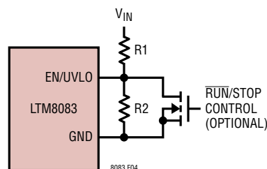
Figure 4. V IN Undervoltage Lockout (UVLO)
