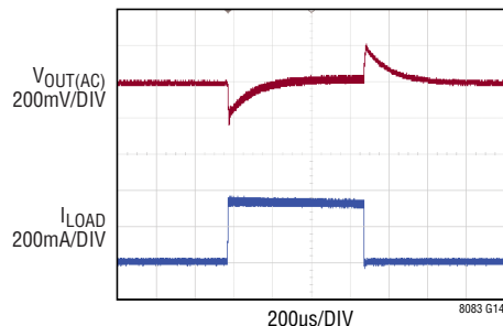
Transient Response from 12V IN to 12V OUT
