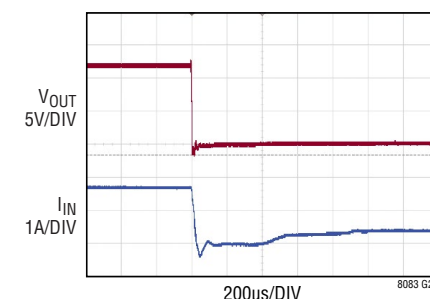
Short-Circuit with 12V_{IN} and 12V_{OUT} at I_{OUT} = 1.5A
