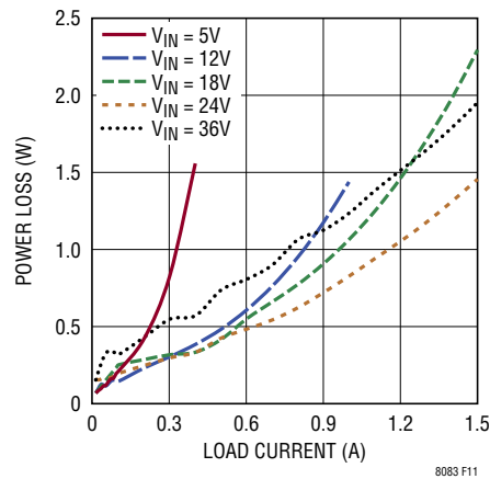
Figure 11. Power Loss at 18V OUT
