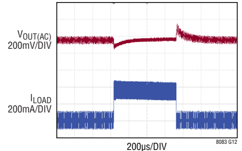
Transient Response from 36V IN to 5V OUT
