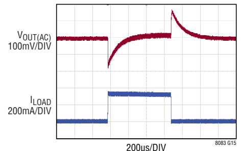
Transient Response from 24V IN to 12V OUT
