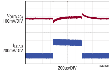
Transient Response from 24V IN to 5V OUT
