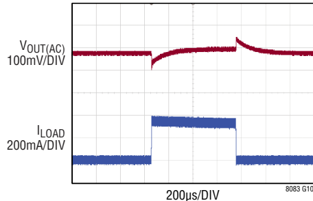
Transient Response from 12V IN to 5V OUT
