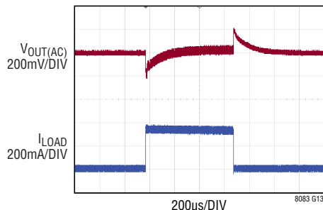
Transient Response from 6V IN to 12V OUT
