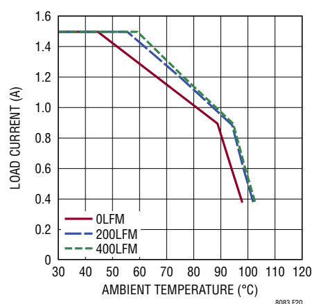
Figure 20. 36V to 36V Derating Curve, No Heat Sink
