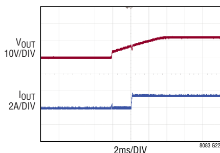
Start-Up with 36V_{IN} and 12V_{OUT} at I_{OUT} = 1.5A
