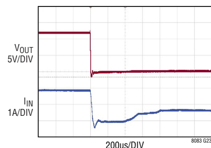
Short-Circuit with 6V_{IN} and 12V_{OUT} at I_{OUT} = 0.8A
