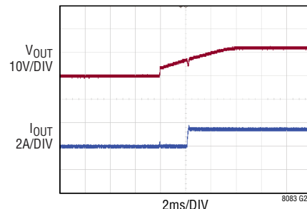
Start-Up with 24V_{IN} and 12V_{OUT} at I_{OUT} = 1.5A
