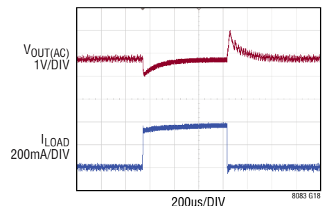
Transient Response from 36V IN to 36V OUT
