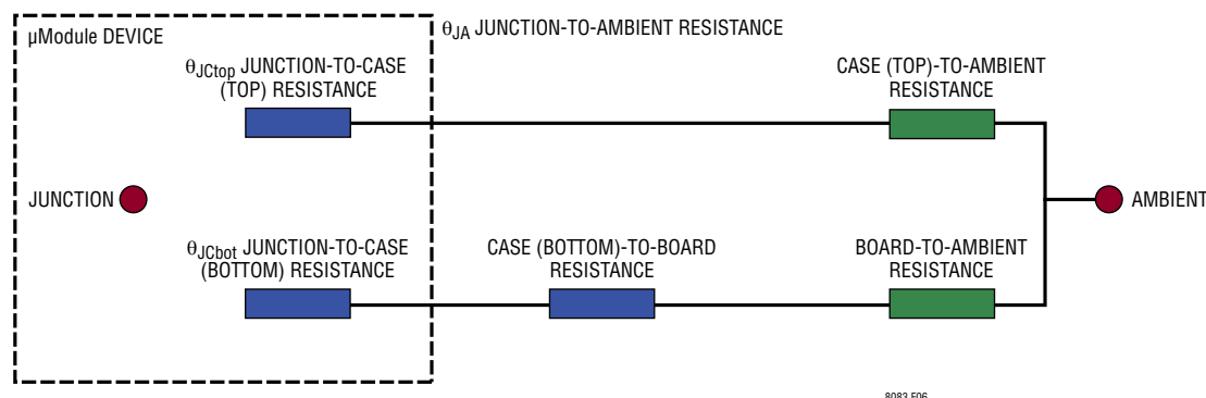
Figure 6. Graphical Approximation of the Thermal Coefficients, Including JEDEC-51-12 Terms
