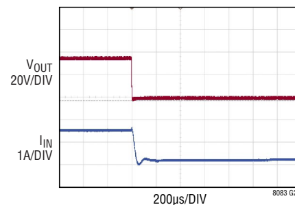
Short-Circuit with 24V_{IN} and 36V_{OUT} at I_{OUT} = 1A
