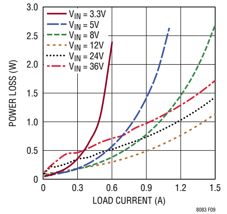
Figure 9. Power Loss at 8V OUT
