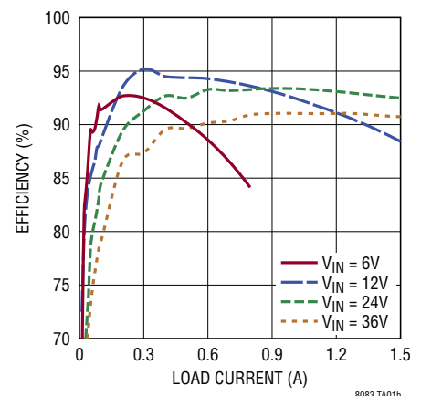
Efficiency at 12V Output
