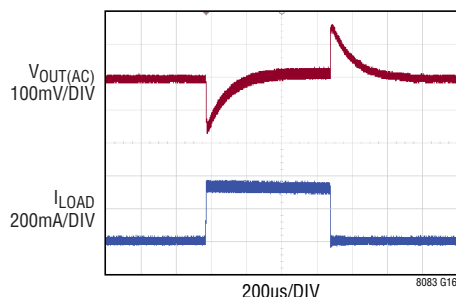
Transient Response from 36V IN to 12V OUT
