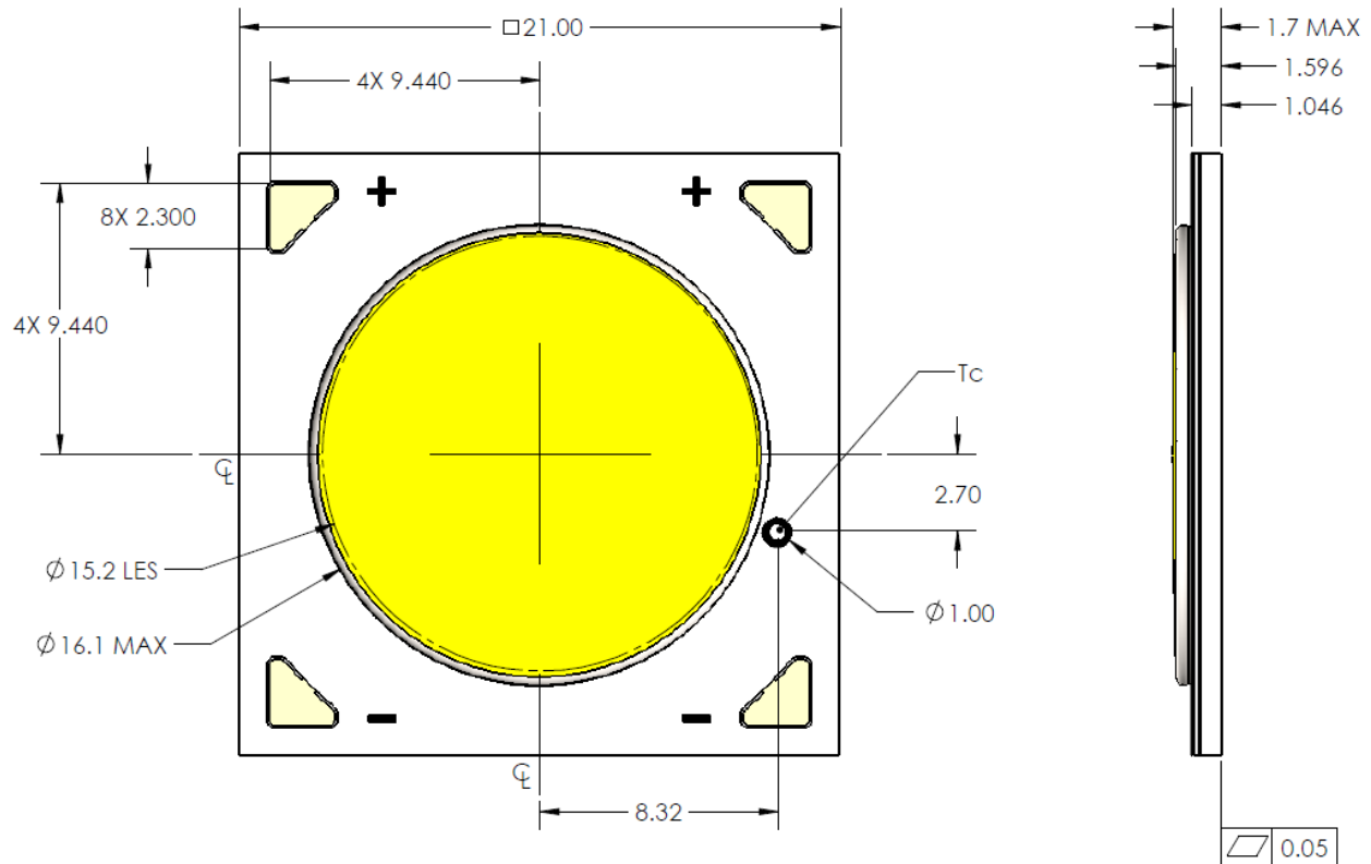
Figure 10: Drawing for V15 Arrays
