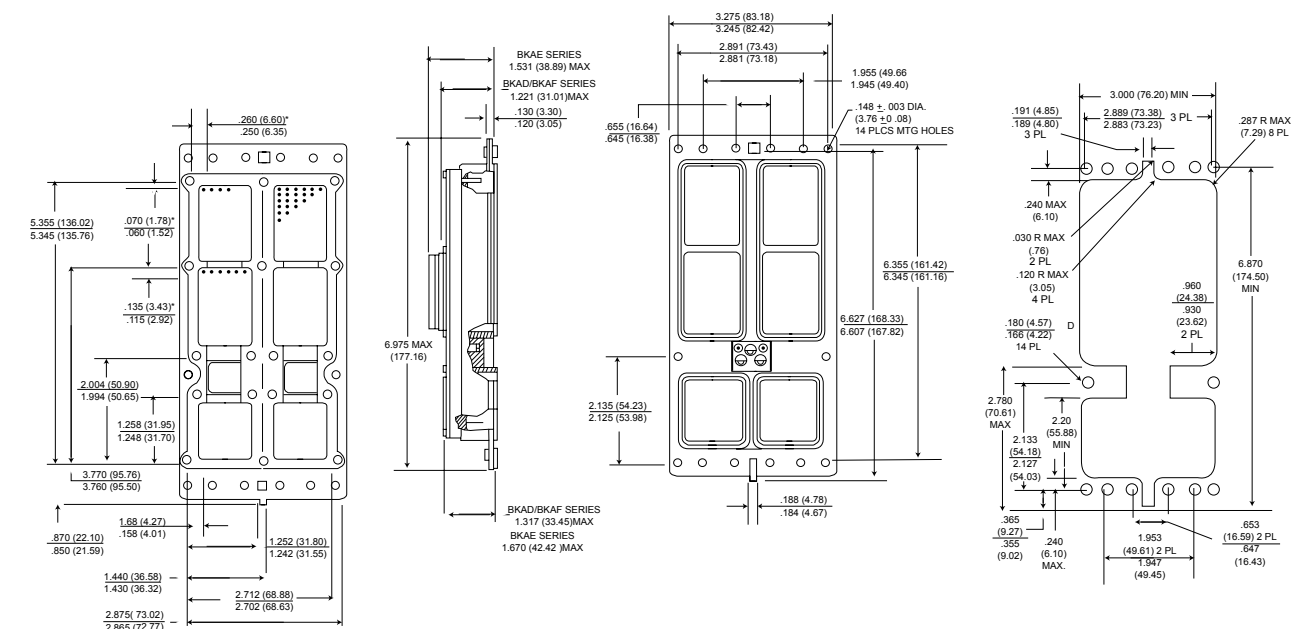
Retainer Plate
