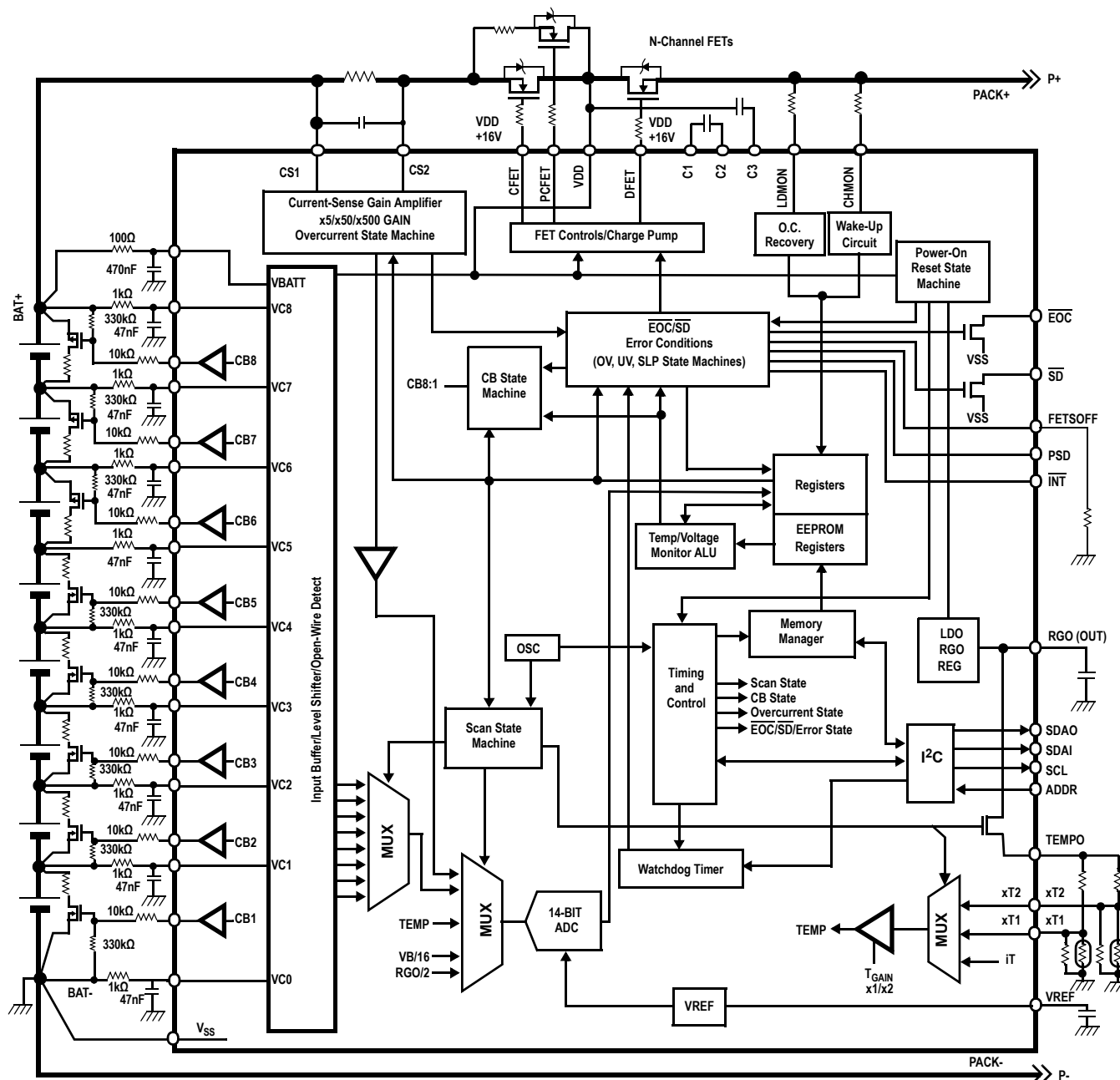
Figure 2. Block Diagram
