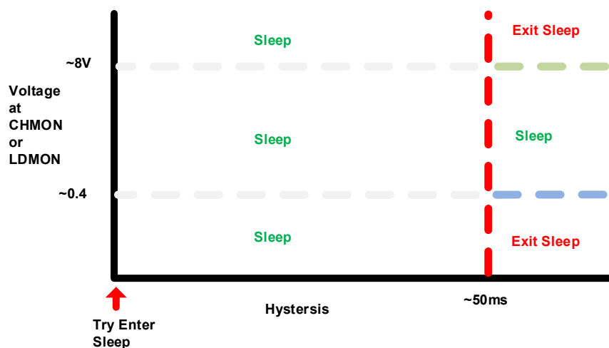
Figure 45. SLEEP Qualification
