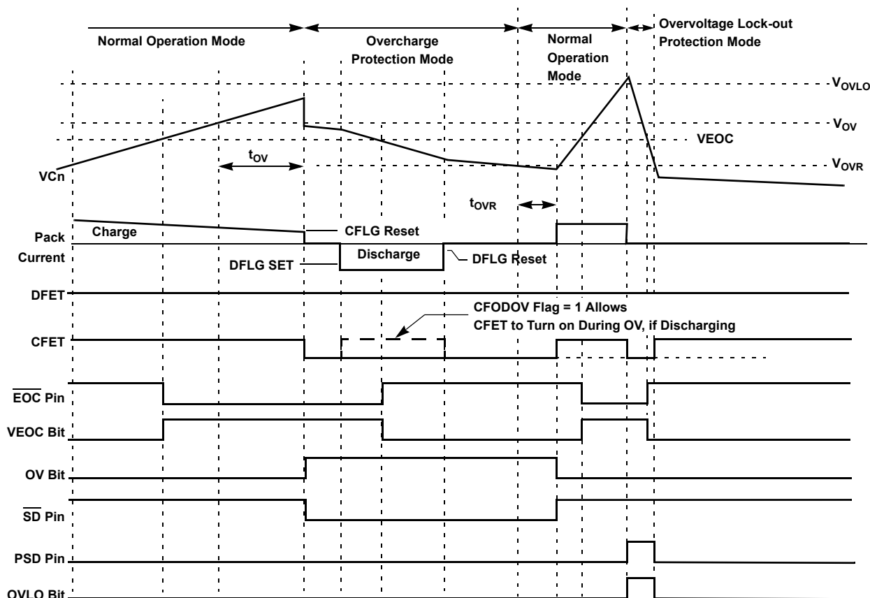
Figure 65. OV Detection/Response
