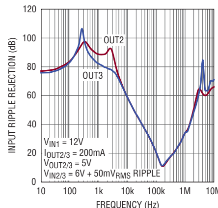
LD0s: Input Ripple Rejection
