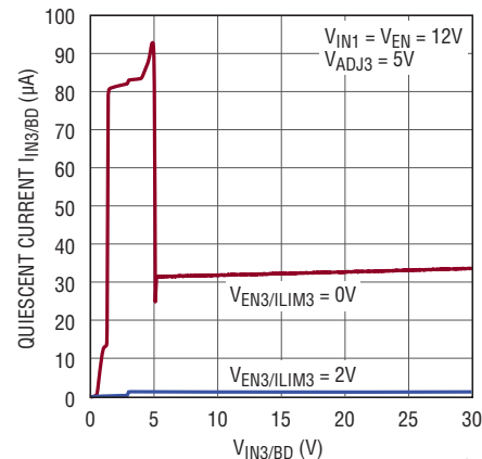
LD0s: 5V Quiescent Current IN3/BD
