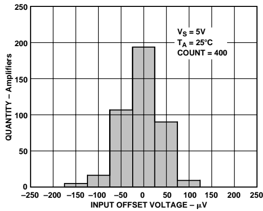
TPC 2. Input Offset Voltage Distribution
