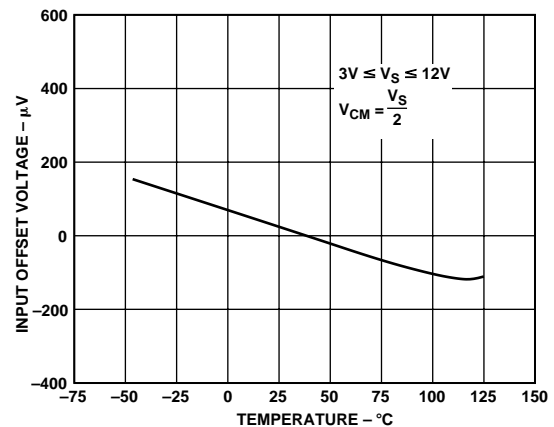
TPC 6. Input Offset Voltage vs. Temperature
