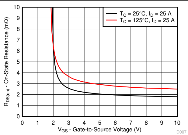
Figure 4-7. On Resistance vs Gate Voltage
