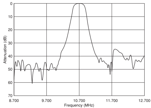
SFECF10M7EA00S0-R0
