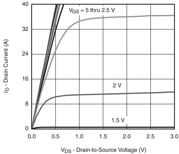
V_{GS} = 5 thru 2.5 V Output Characteristics
