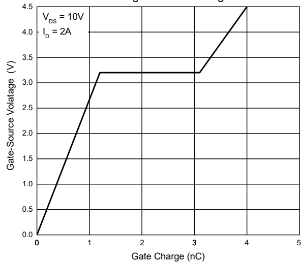
Fig. 6 - Gate Charge
