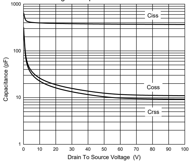
Fig. 5 - Capacitance Characteristics
