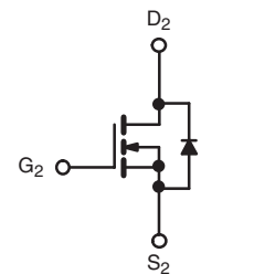
N-Channel MOSFET
