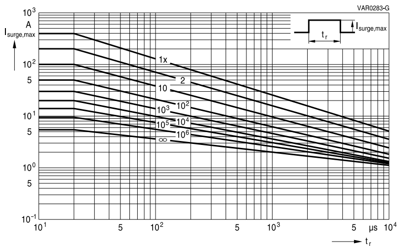
CT1210L8G ... K20G
