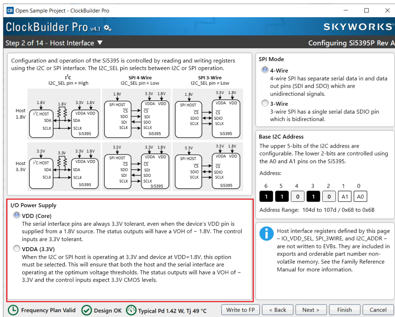
Figure 73. Determine the Value of IO_VDD_SEL Bit Written to Device
