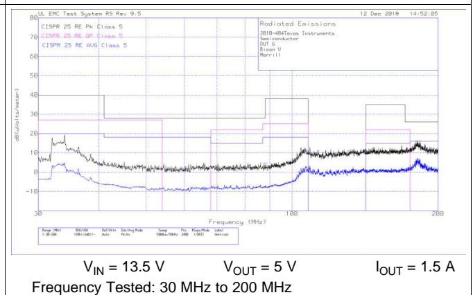
Figure 39. Radiated EMI Bicon Vertical vs. CISPR25 Limits
