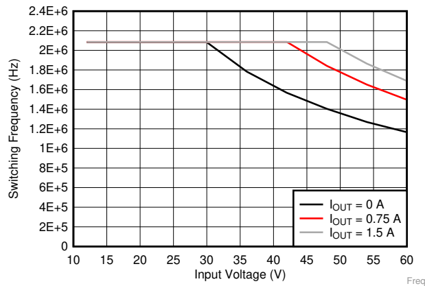
Figure 17. Switching Frequency vs Input Voltage V_{OUT} = 5\text{ V}
