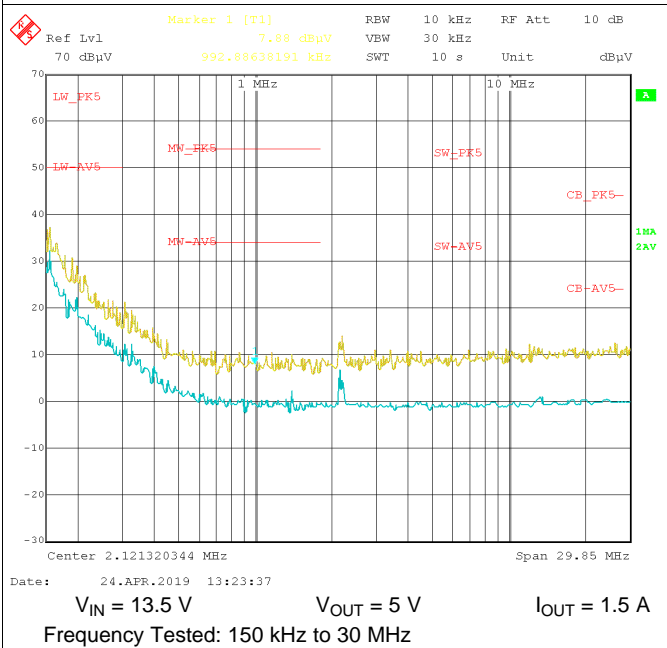
Figure 36. Conducted EMI vs. CISPR25 Limits (Yellow: Peak Signal, Blue: Average Signal)
