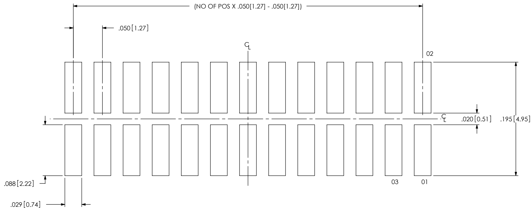
FIG. 2 (-113 POSITION SHOWN) (ALL DIMENSIONS ARE SYMMETRIC ABOUT THE CENTERLINE)
