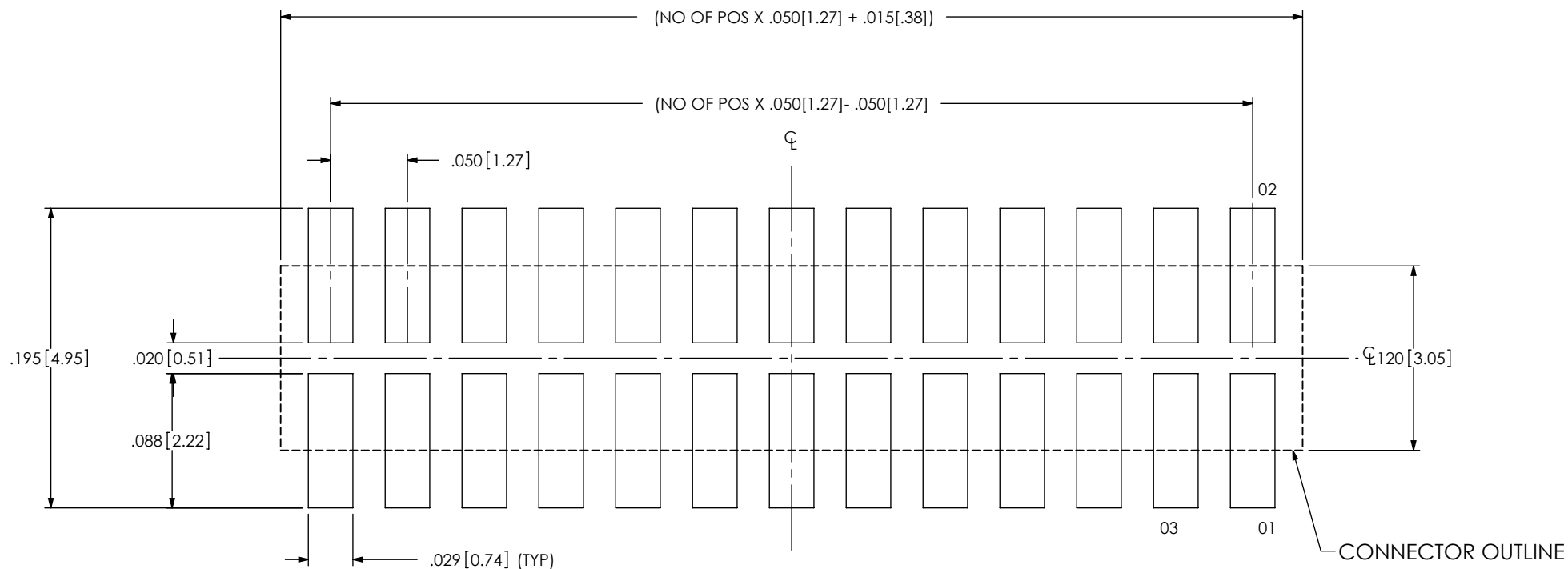
FIG 1 (-113 POS SHOWN) (ALL DIMENSIONS ARE SYMMETRIC ABOUT THE CENTERLINE)
