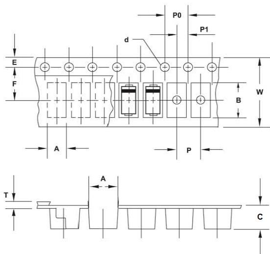
DO-214AB(SMC) - Tape carrier
