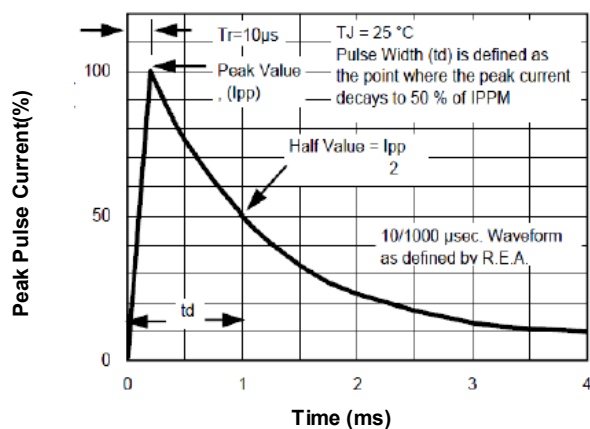
Fig 5. Pulse Waveform
