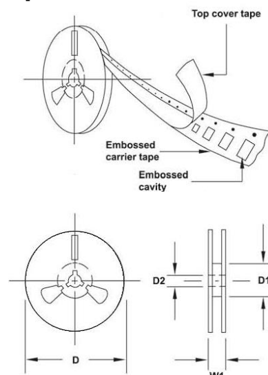
DO-214AA(SMB) - Reel
