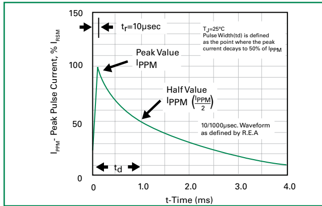
Figure 4 - Pulse Waveform
