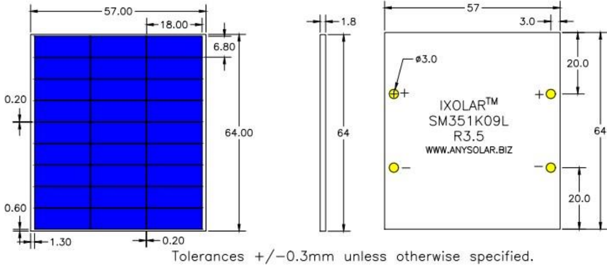
Front-side View details
