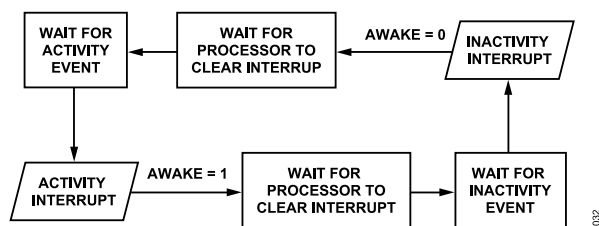
Figure 41. Flowchart Illustrating Activity and Inactivity Operation in Linked Mode
