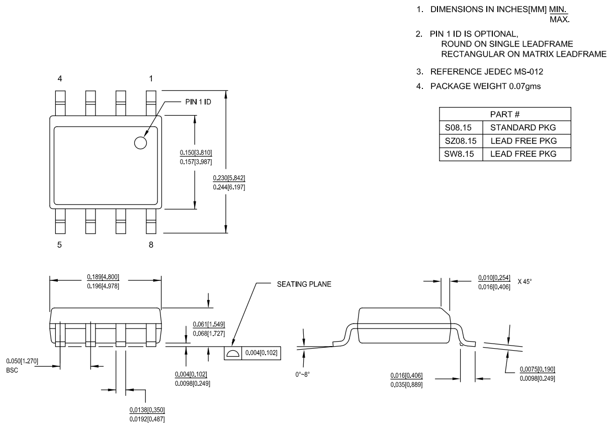
Figure 9. 8-pin SOIC (150 Mils) Package Outline, 51-85066
