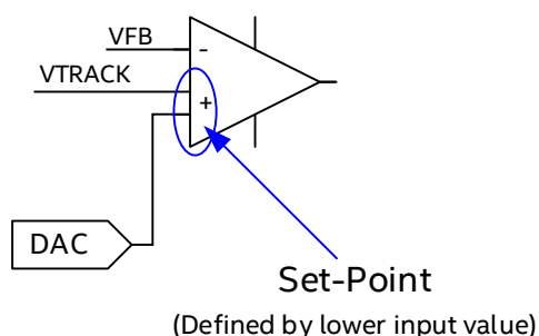
Figure 10: VTRACK Circuitry
