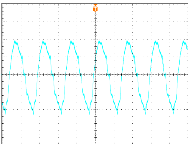
Output voltage ripple at nominal input voltage and max load current (30mV/div, 2us/div) Load cap: 10μF, tantalum capacitor and 1μF ceramic capacitor. Bandwidth: 20MHz.
