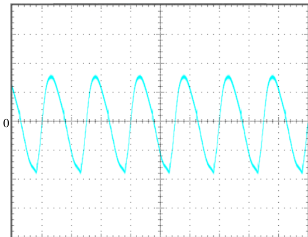
Output voltage ripple at nominal input voltage and max load current (20mV/div, 2us/div) Load cap: 10 \mu F, tantalum capacitor and 1 \mu F ceramic capacitor. Bandwidth: 20MHz.
