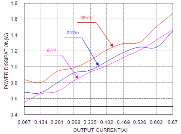
Power dissipation vs. load current at 25°C.
