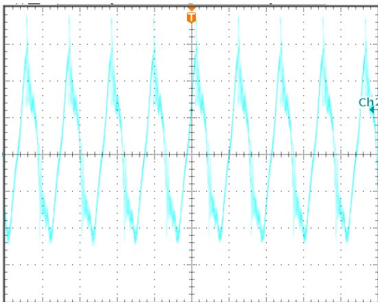
Output voltage ripple at nominal input voltage and max load current (5mV/div, 2us/div) Load cap: 10µF, tantalum capacitor and 1µF ceramic capacitor. Bandwidth: 20 MHz.
