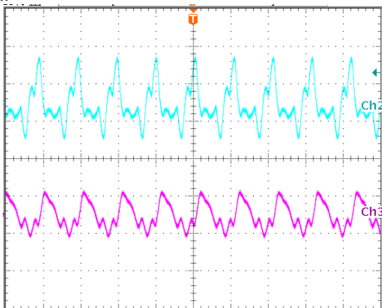
Output voltage ripple at nominal input voltage and max load current Top trace +12V, 10 mV/div, Bottom trace -12V, 20mV/div, 2us/div. Load cap: 10μF, tantalum capacitor and 1μF ceramic capacitor. Bandwidth: 20 MHz.
