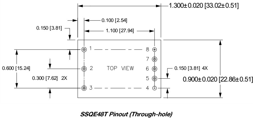
SSQE48T Pinout (Through-hole)
