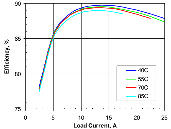
Figure 3. Efficiency vs. load current and ambient temperature for SSQE48T25025 converter mounted vertically with V_{in}=48\text{V} and air flowing from pin 1 to pin 3 at a rate of 200LFM (1.0m/s).
